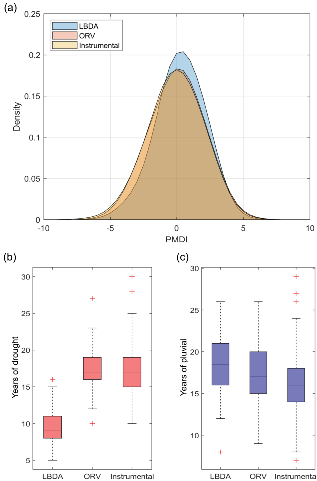
Figure 6. (a) Probability distribution functions for all gridded reconstructed PMDI values for the ORV and LBDA networks. (b) Boxplot of the number of drought (PMDI \leq -2.0 ) years between LBDA and ORV. (c) Boxplot of the number of pluvial (PMDI \geq 2.0 ) years between LBDA and ORV.
